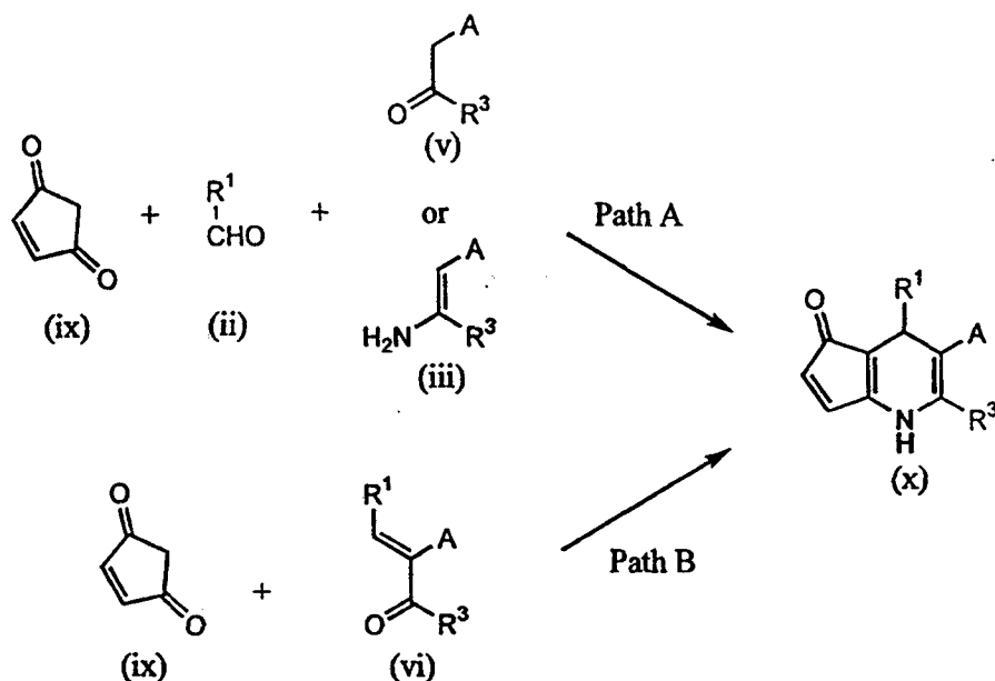
Scheme 3
