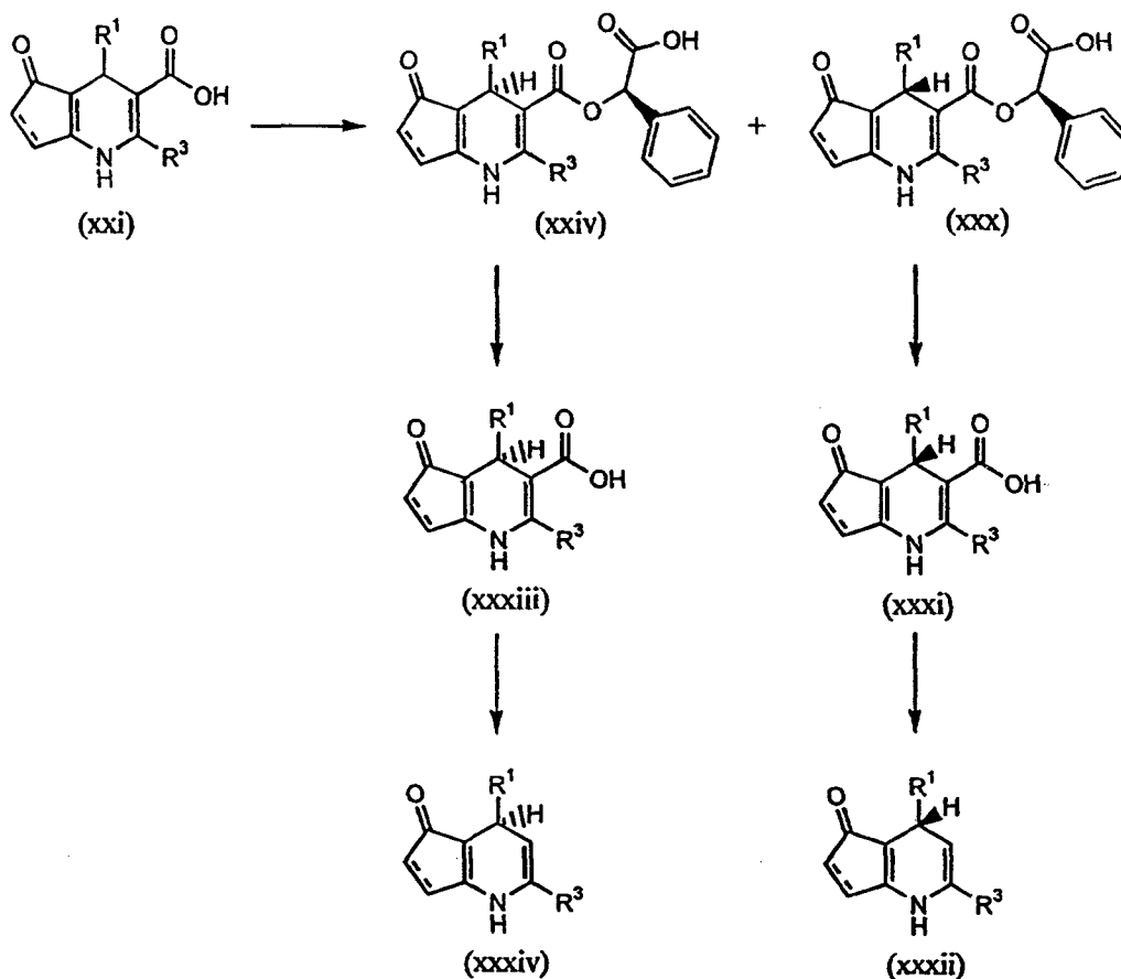
Scheme 9
