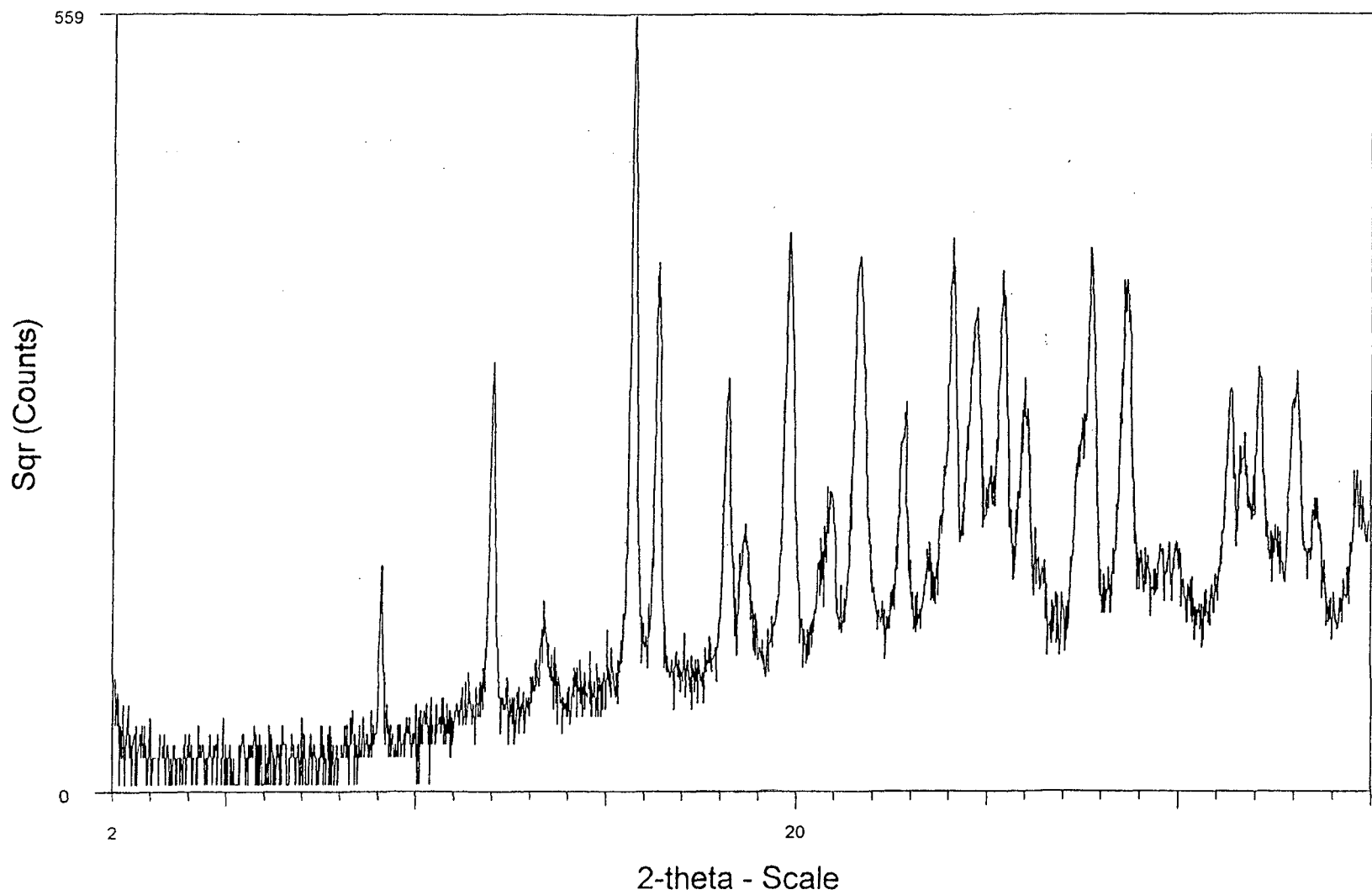
Figure II. X-Ray Powder Diffraction Pattern of Hydrochloride Hydrate
