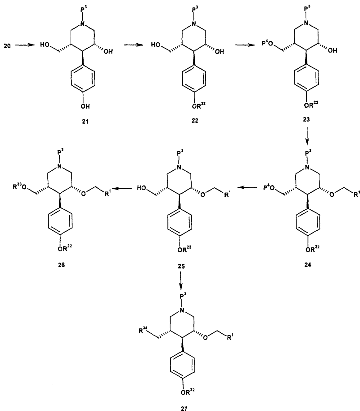
Scheme 4:
