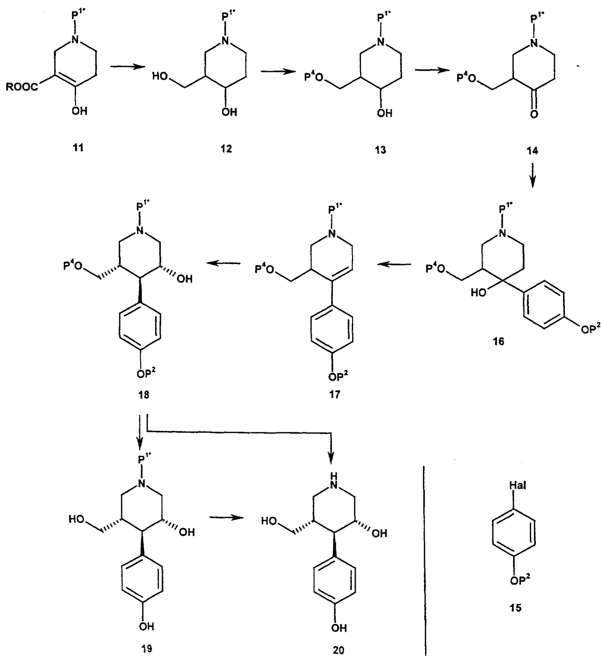
Scheme 3:
