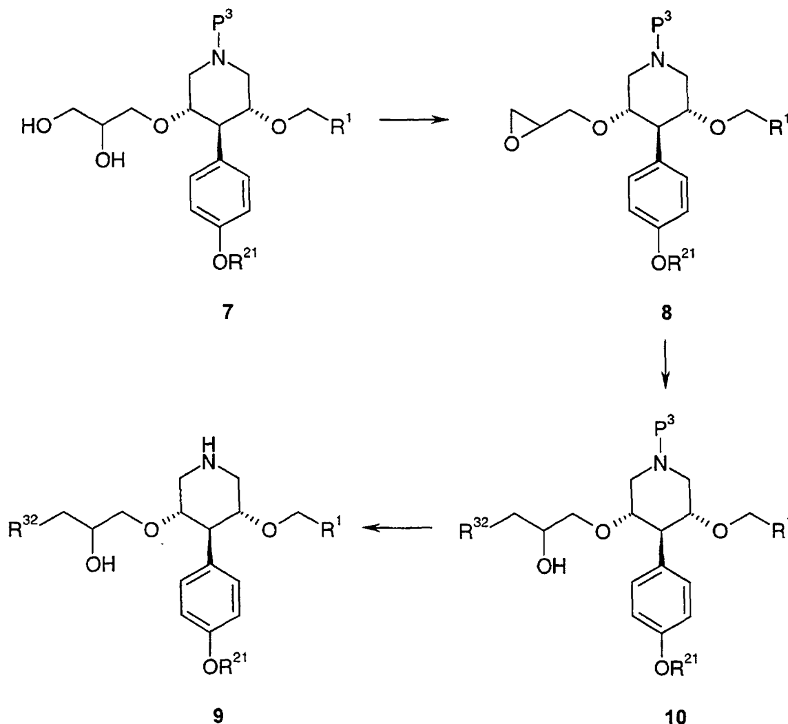
Scheme 2:
