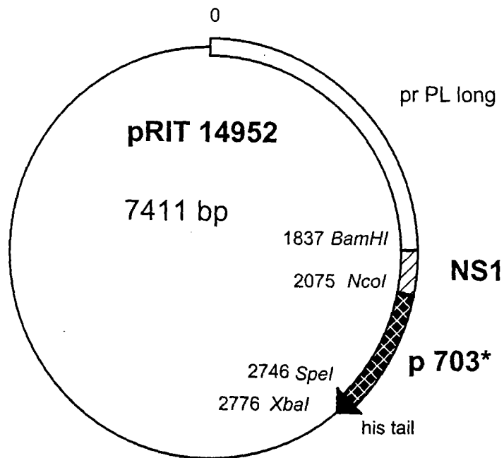
Figure 5: Plasmid map of pRIT 14952
