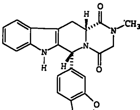
(6R,12aR)-2,3,6,7,12,12a-hexahydro-2-methyl-6-(3,4-methylenedioxyphenyl)pirazino[2',1':6,1]pindo[3,4-b]indol-1,4-dione
