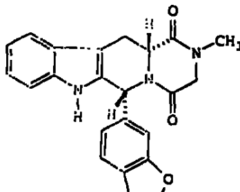
(6R,12aR)-2,3,6,7,12,12a-hexahidro-2-metil-6-(3,4-metilendioxifenil)pirazino[2',1':6,1]pirido[3,4-b]indol-1,4-diona
