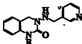
Figure 3. Structure of the reduced form and R-768.
