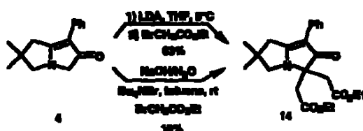
Scheme 6: Alkylation of 4
