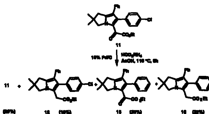
Scheme 9: deoxygenation of 11
