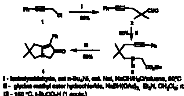
Scheme 3: Synthesis and thermolysis of \alpha -acetylenic amino ester 5
