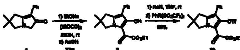
Scheme 8: Suzuki coupling
