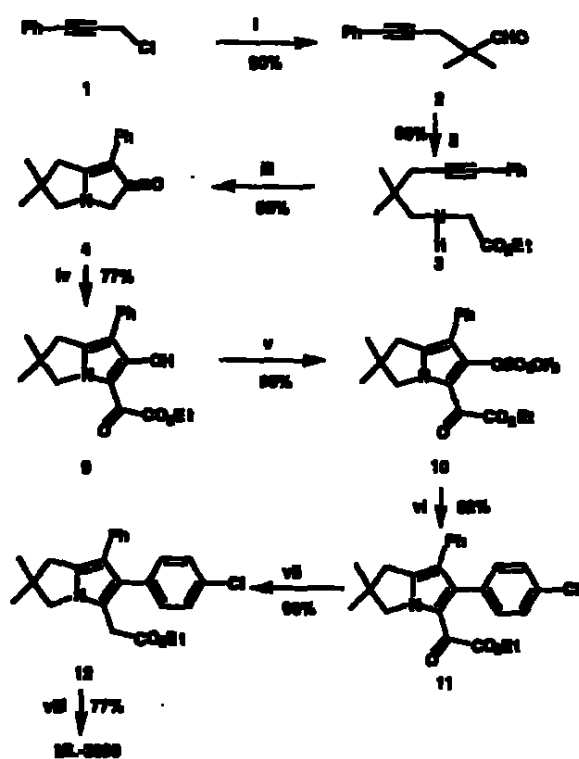
Scheme 11: Synthesis of ML-3000
