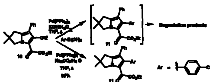
Scheme 8: Suzuki coupling
