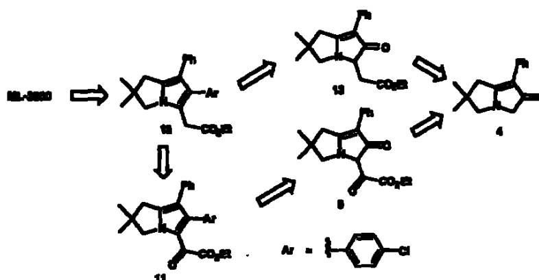
Scheme 5: Second approach to ML-3000
