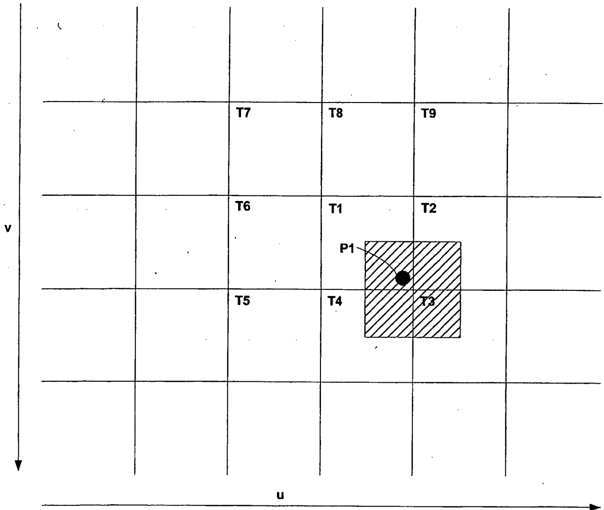
FIG. 2B - Prior Art Bilinear Filtering
