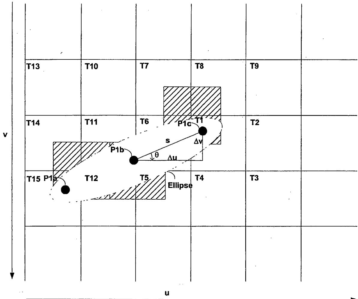
FIG. 2D - Prior Art Anisotropic Filtering
