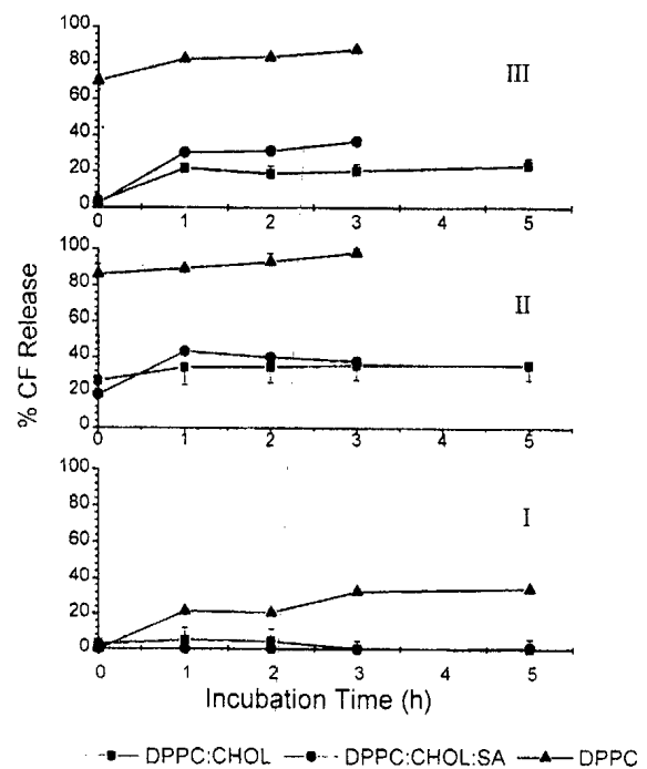
Fig. 3. Release of encapsulated carboxyfluorescein from DPPC-based liposomes after incubation at 37°C in the presence of: (I) pancreatin, (II) 10 mM sodium cholate and (III) 10 mM sodium taurocholate. Each point is the mean of at least four experiments (bars represent SD values). Key: triangles, plain lipid; squares, lipid:chol; circles, lipid:chol:SA.
