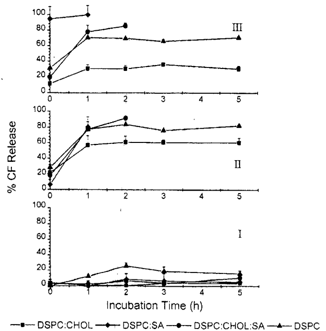
Fig. 4. Release of encapsulated carboxyfluorescein from DSPC based liposomes after incubation at 37°C in the presence of: (I) pancreatin, (II) 10 mM sodium cholate and (III) 10 mM sodium taurocholate. Each point is the mean of at least four experiments (bars represent SD values). Key: triangles, plain lipid; squares, lipid:chol; circles, lipid:chol:SA; diamonds.
