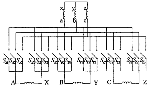
Fig. 3. Control of winding connections using matrix converter.
