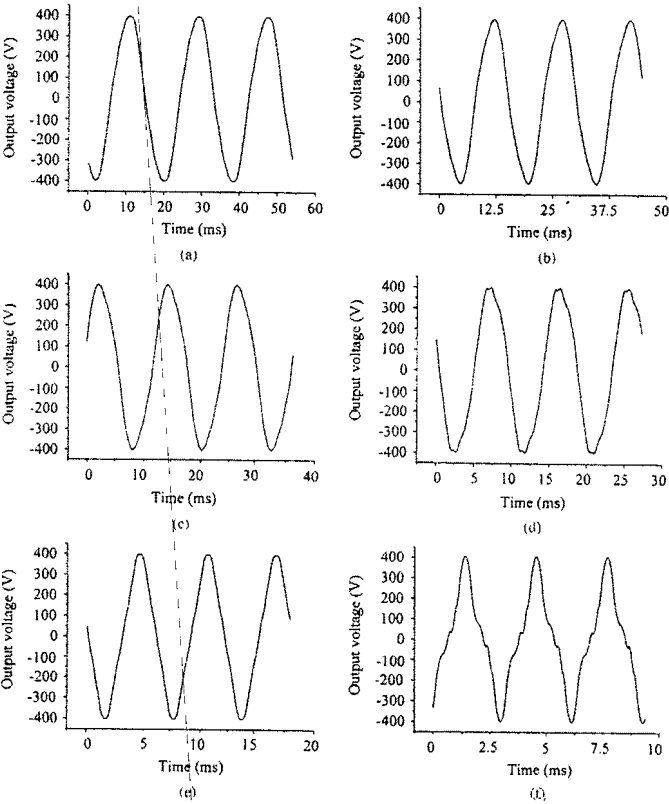
Fig. 6. Simulated output voltages in different modes. (a) 300 rpm. (b) 360 rpm. (c) 450 rpm. (d) 600 rpm. (e) 900 rpm. (f) 1800 rpm.
