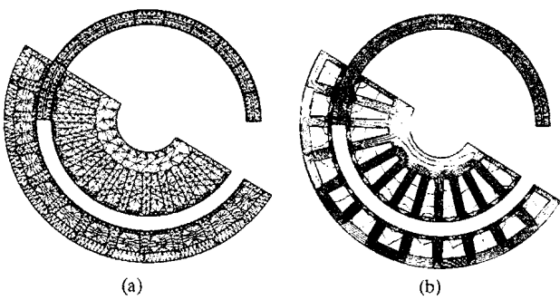
Fig. 4. CFT-TS-FEM analysis. (a) Mesh. (b) Magnetic field distribution.
