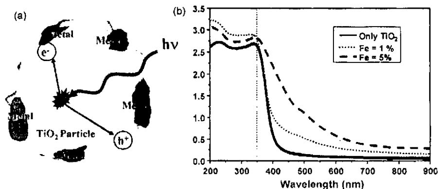
Fig. 16. (a) Electrons capture by a metal in contact with a semiconductor surface. (b) UV-vis spectra of iron-doped titania catalysts.
