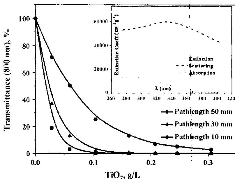
Fig. 6. Transmittance and extinction coefficient (inset) of \text{TiO}_2 Degussa P-25, at pH 6, suspension in water.
