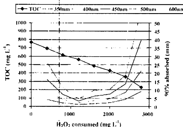
Fig. 22. Experiment in pilot-plant. \alpha -Methyl phenyl glycine = 1 g L -1 ; C Fe = 1 mM, V = 75 L. Optical pathlength, after which 90% of radiation is absorbed. Initial sample not shown, because the contaminant does not absorb at wavelengths above 300 nm.
