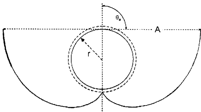
Fig. 11. Schematic drawing of CPC with a semi-angle of acceptance of 90°.
