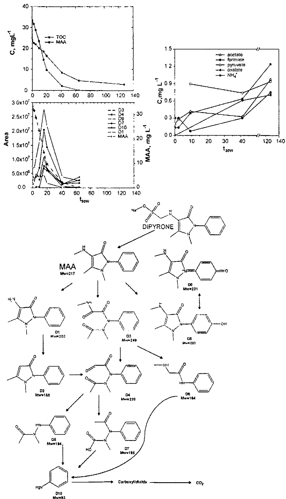
Fig. 13. (a) Dipyrone degradation (dipyrone is readily hydrolysed to 4-methylaminoantipyrine) kinetics during solar photocatalysis, kinetics of the most important DPs formed, evolution of the main carboxylic acids and inorganic species detected. (b) Degradation pathway.
