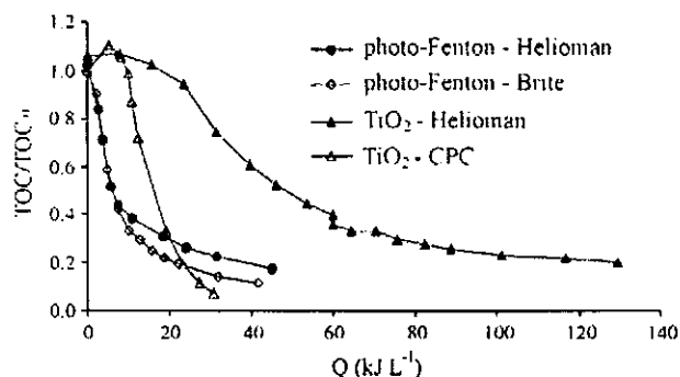
Fig. 23. Degradation of mixture of commercial pesticides. \text{TOC}_0 = 100 \text{ mg L}^{-1} , Photo-Fenton: \text{Fe} = 20 \text{ mg L}^{-1} , \text{H}_2\text{O}_2 consumption = 1.5 \text{ g L}^{-1} ; \text{TiO}_2 : \text{TiO}_2 = 0.2 \text{ g L}^{-1} , \text{Na}_2\text{S}_2\text{O}_8 consumption = 2.5 \text{ g L}^{-1} .
