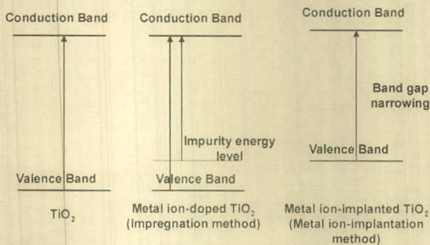
Fig. 18. Scheme of TiO 2 band structures, chemically ion-doped TiO 2 and physically ion-implanted TiO 2 .
