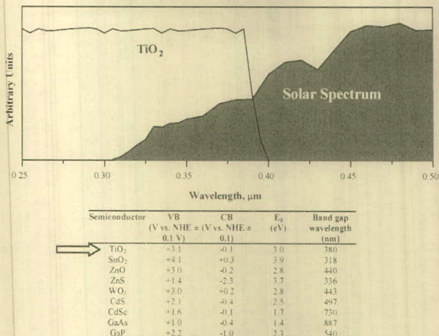
Fig. 3. Band position (water at pH 1) for some common semiconductor photocatalyst: VB (valence band), CB (conduction band), E g (band-gap energy). TiO 2 absorption spectrum compared with solar spectrum is also shown.
