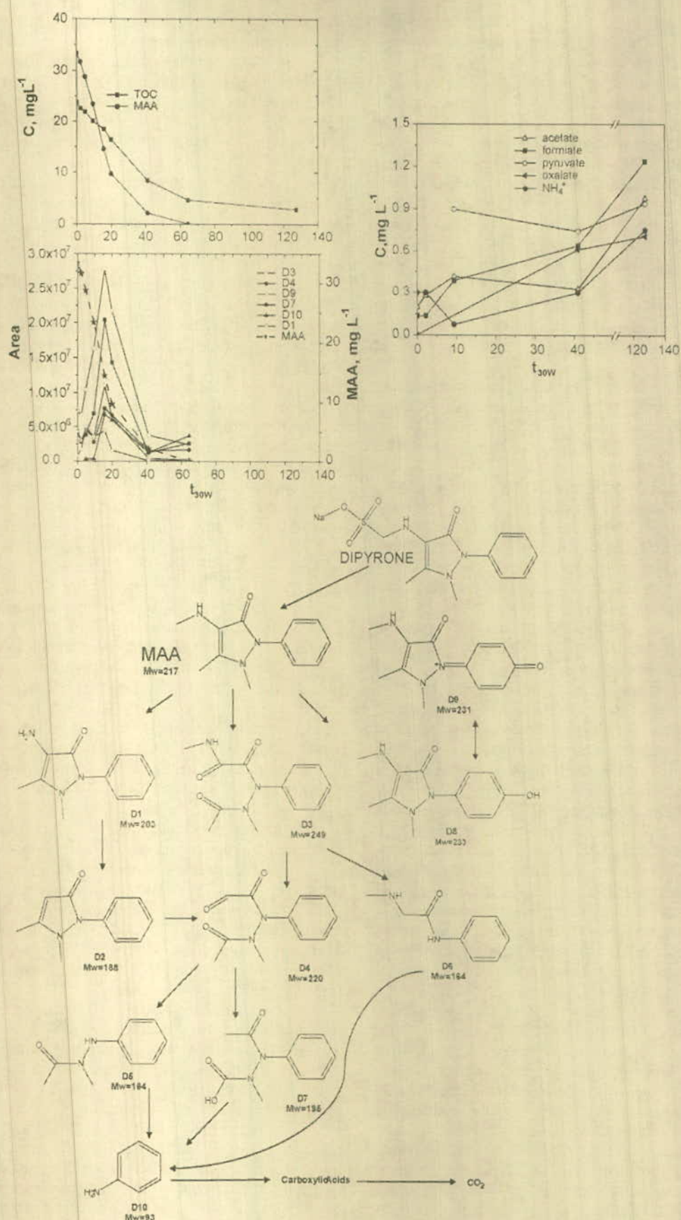
Fig. 13. (a) Dipyrone degradation (dipyrone is readily hydrolysed to 4-methylaminoantipyrine) kinetics during solar photocatalysis, kinetics of the most important DPs formed, evolution of the main carboxylic acids and inorganic species detected. (b) Degradation pathway.
