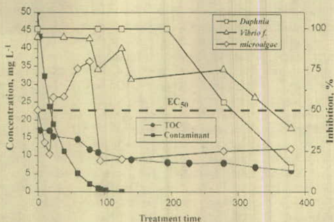
Fig. 14. Degradation mineralization and evolution of toxicity (right axis) during a photocatalytic treatment in a pilot plant.
