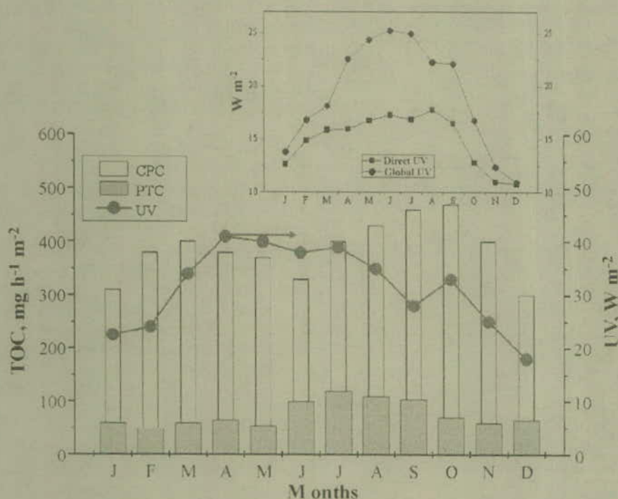
Fig. 8. TOC disappearance reaction rate for a concentrating (PTC) and a non-concentrating (CPC) collector system [24]. The mean value of global UV radiation during the experimental periods is also shown. Average UV direct and UV global (direct + diffuse) irradiance for each month of the year at Plataforma Solar de Almería is shown in the inset.
