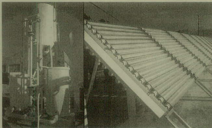
Fig. 15. Photographs of solar detoxification demonstration plant constructed in "SOLARDETOX" project at HIDROCEN (Madrid, Spain). Left: TiO 2 separation system. Right: compound parabolic collector.
