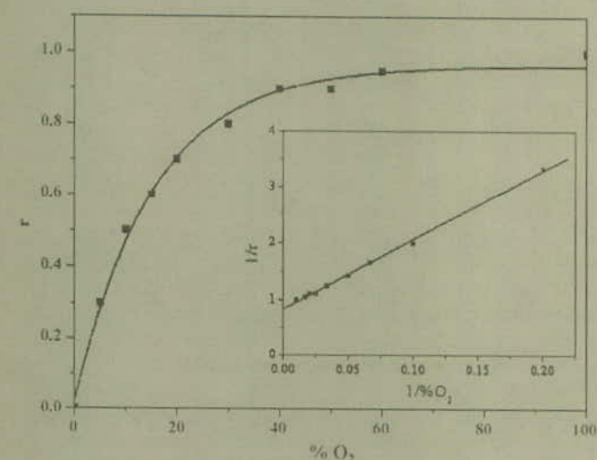
Fig. 9. Plots of initial relative rate ( r ) vs. concentration of oxygen ( \%O_2 ) and 1/r vs. 1/\%O_2 .
