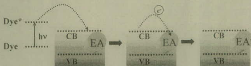
Fig. 19. Steps of excitation with a sensitizer in the presence of an adsorbed organic electron acceptor (EA).
