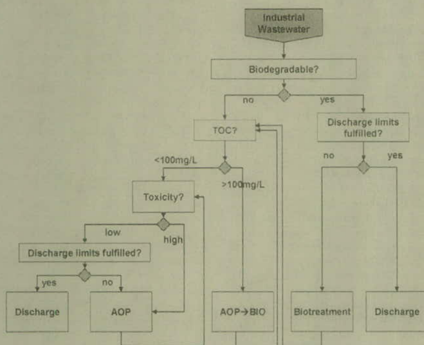
Fig. 24. Decision scheme for selecting the appropriate treatment train.
