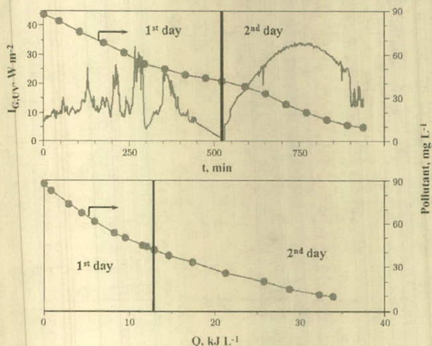
Fig. 5. Example of solar degradation experiments depicted vs. t (up) and vs. Q (down). Solar UV irradiance throughout the experiment is also shown.
