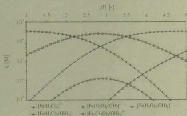
Fig. 21. Ferric iron species present in aqueous solution at different pH at a concentration of 20 \text{ mg L}^{-1} , calculated with equilibrium constants from [166]. T = 20^\circ \text{C} .
