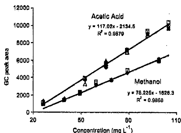
Fig. 3. Calibration curves for methanol with: no acetic acid ( \blacklozenge ), 80 \text{mg L}^{-1} acetic acid ( \square ), and for acetic acid with: no methanol ( \blacklozenge ), 60 \text{mg L}^{-1} methanol ( \square ) and 100 \text{mg L}^{-1} methanol ( \triangle ).
