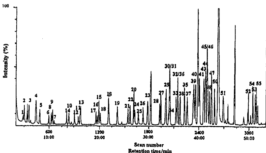
Fig. 4. Full-scan GC/MS separation on a 60m×0.25mm ID×1.4 μm film thickness DB-VRX column, of 56 volatile organic contaminants obtained by purge-and-trap headspace sampling from an aqueous sample. Reprinted by permission of the Royal Society of Chemistry from [32].
