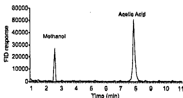
Fig. 1. HS-SPME-GC-FID chromatogram for separation of methanol (2.5 min) and acetic acid (7.8 min).
