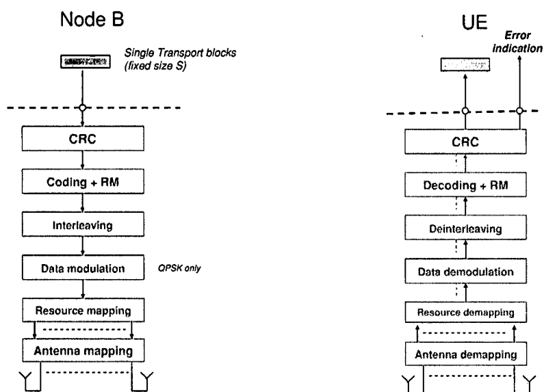
Figure 5.4.1.2: BCH physical-layer model
