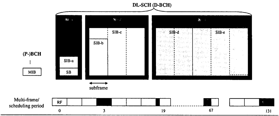
Fig. x System information structure and typical scheduling example
