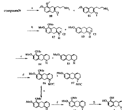
Scheme 2. Synthesis of 4 . Reagents and conditions: (a) Na/EtOH, reflux, 1 h; (b) MeOH, 57% HCl, reflux, 4 h; (c) NaCNBH 3 ; (d) (BOC) 2 O, Et 3 N, DMAP; (e) TFA, CH 2 Cl 2 ; (f) CH 2 CH 2 CHO, 1 bar H 2 , 10% Pd/C, n -propanol, rt, 2 h; (g) HBr 48%, 3 h.
