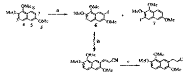
Scheme 1. Synthesis of 4 . Reagents and conditions: (a) n -BuLi, THF, -78 °C to rt, overnight; -78 °C, 1 h, 10 min; (b) CH 2 =CH-CN, Pd(OAc) 2 , Et 3 N, CH 3 CN, 120 °C, 3 days; (c) 10% Pd/C, 4 bar H 2 , rt, overnight.
