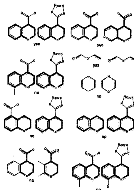
Figure 2. Examples of pairs of molecules where the extracted fragment-pair would pass (yes) or fail (no) the filters for algorithm A. The filters are meant to detect one-to-one replacements of a single chemical group.
