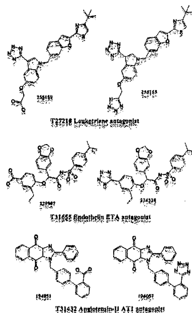
Figure 8. Examples from the MDDR where a carboxylate \rightleftharpoons tetrazole replacement is made in different therapeutic categories.
