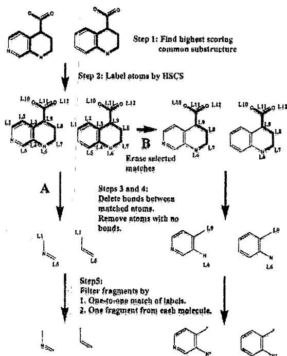
Figure 1. A schematic diagram of how replaced groups are parsed as a fragment-pair from a pair of molecules. There are two alternative paths (marked "A" and "B") depending on whether match atoms in rings or other groups are declared unmatched after Step 2 (see text). Steps 3–5 are the same thereafter. Bonds connecting match atoms are shown as bold. At the bottom of the figure, the match atoms remaining after processing are indicated by "*".
