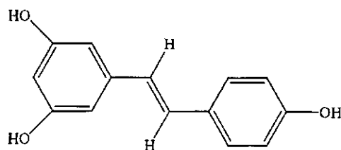
Figure 1. Chemical structure of trans resveratrol.
