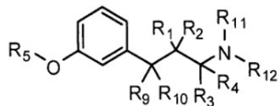
Formula (IIa)
