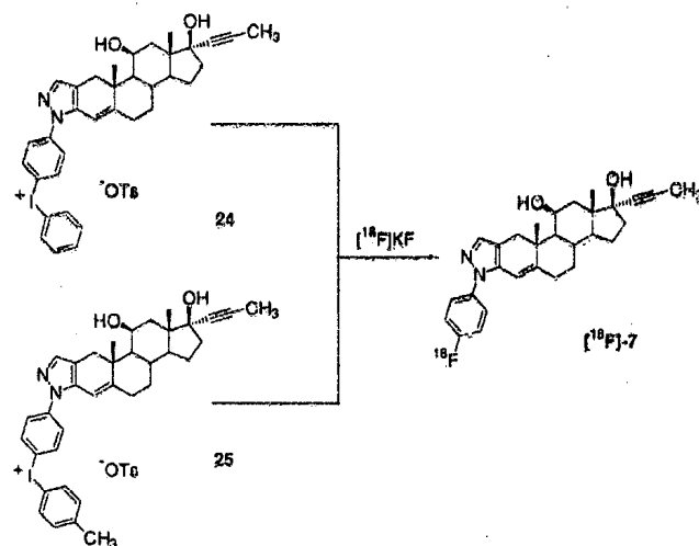
Fig. 8. Radiosynthesis of ^{18}\text{F} -labeled steroid [^{18}\text{F}] -7 via diaryliodonium salts 24 and 25.
