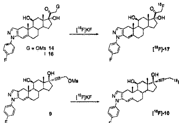
Fig. 7. Radiosynthesis of ^{18}\text{F} -labeled steroids [^{18}\text{F}] -17 and [^{18}\text{F}] -10.
