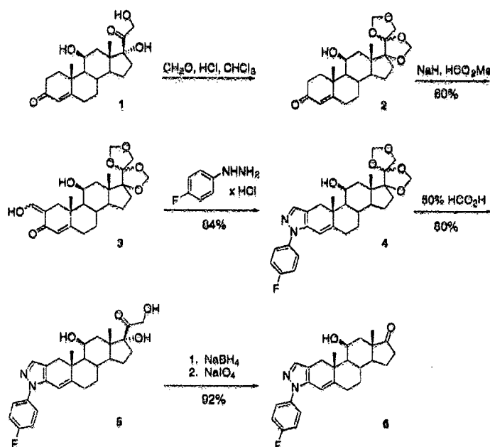
Fig. 2. Synthesis of 2'-(4-fluorophenyl)-11β-hydroxy-androst-4-ene-17-one[3,2- c ]pyrazole 6.
