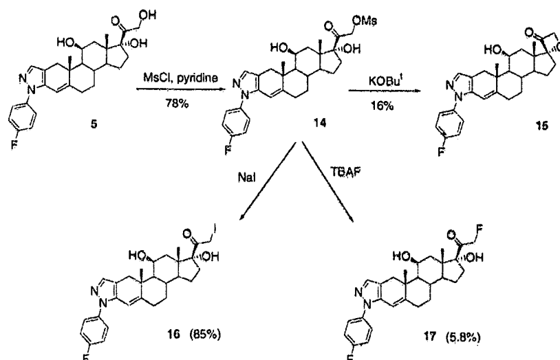
Fig. 4. Synthesis of steroids containing an oxetan-3'-one moiety and modified 1,3-dihydroxyacetone side chains.
