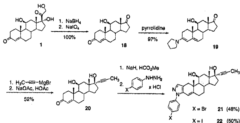
Fig. 5. Synthesis of 4-bromo- and 4-iodophenylpyrazolo steroids 21 and 22.
