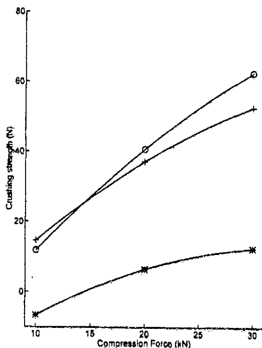
Fig. 3. Prediction of the crushing strength of mannitol MCC tablets as a function of the amount of MCC and the compression force. (MCC: \circ = 65%, + = 75%, * = 90%; HPC 3%, granulation time 5 min, moisture in granulate 4%, water at its medium level).
