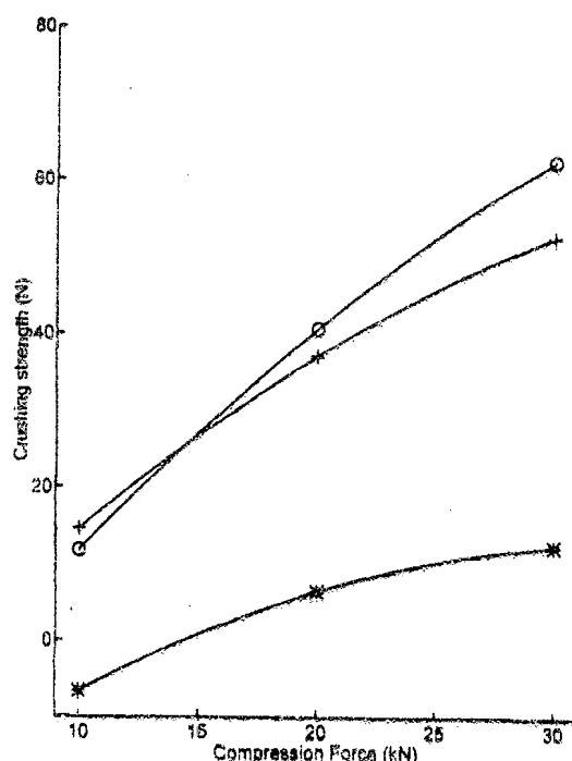
Fig. 3. Prediction of the crushing strength of mannitol MCC tablets as a function of the amount of MCC and the compression force. (MCC: ○ = 65%, + = 75%, * = 90%; HPC 3%, granulation time 5 min, moisture in granulate 4%, water at its medium level).
