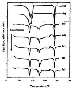
Fig. 12. Differential scanning calorimetry (DSC) curves of aspartame hemihydrate at different pressures: (a) at atmospheric pressure in a conventional DSC cell; (b) at atmospheric pressure in a pressure DSC (PDSC) cell; (c) 100 p.s.i.; (d) 200 p.s.i.; (e) 300 p.s.i.; (f) 400 p.s.i.; and (g) 600 p.s.i. (1 p.s.i. = 6.9 kPa) [179], reproduced with the permission of Elsevier Science.
