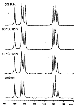
Fig. 11. Solid-state ^{13}\text{C} -NMR spectra of LY97902 tartrate ((+)-3-(4-(benzylthio)-1,2,5-dioxolyl-4-yl)-5-hydroxy-2,2-diphenyl-methoxydiphenylacetate) after storage at 0% humidity and before and after drying at elevated temperatures [75], reproduced with the permission of the American Pharmaceutical Association.
