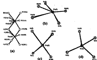
Fig. 10. In hydrated cromolyn sodium, coordination environment of: (a) the first (ordered) sodium ion, Na(1), shown in two neighboring unit cells (A and B); and the second (disordered) sodium ion at its three partially occupied sites, (b) Na(2) to Na(3), and (d) Na(4). The striped circles represent the sodium sites. The open circles represent the oxygen atoms coordinated to Na(1). The dotted (gray) circles represent the oxygen atoms coordinated to Na(2), Na(3), or Na(4) [71], reproduced with the permission of the American Pharmaceutical Association.
