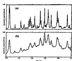
Fig. 8. A partial comparison of (a) a synchrotron pattern of polymorph II of roxibfan, collected using a wavelength of 1.00000 Å with (b) a conventional X-ray diffraction pattern using \text{CuK}\alpha radiation in a region where there are many overlapping peaks. The patterns are plotted as a function of Q = 2\pi d \sin \theta / \lambda to remove the effects of different wavelengths [66], reproduced with the permission of the American Pharmaceutical Association.
