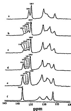
Fig. 9. Resonance signal of the phenyl carbon (C-15) attached to the side chain in the ^{13}\text{C} -CP-MAS NMR spectra of neotame anhydride: (a) sample generated by placing the original monohydrate under vacuum ( -1 Torr) for 3 days; (b–e) sample after being sealed in a jar for 2, 4, 6 and 8 days, respectively; (f) sample after being exposed to a relative humidity environment of 84% for 12 days [29], reproduced with the permission of the American Chemical Society.
