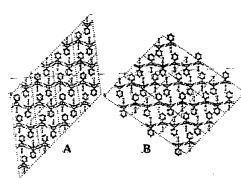
Fig. 6. Comparison of the crystal structure of primidone A (A) versus the most likely packing arrangement, form B (B) [55], reproduced with the permission of Elsevier Science.
