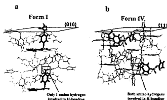
Fig. 7. Possible binding interaction of ethanedisulfonamide in the fastest growing faces of (a) form I and (b) form IV of sulfathiazole ([9], reproduced with the permission of Elsevier Science).
