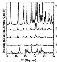
Fig. 13. Powder X-ray diffraction patterns of aspartame hemihydrate: (a) theoretical powder pattern calculated from the crystal structure of aspartame hemihydrate (form I) determined by Hünig et al. (1985) [91]; (b) experimental powder pattern of the ball-milled aspartame hemihydrate (form I); (c) experimental powder pattern of aspartame hemihydrate that had been heated for 30 min at 160°C in the presence of steam (form I); (d) experimental powder pattern of aspartame hemihydrate after compression at 230 MPa for 1 min (form II); and (e) aspartame hemihydrate as received (form II) [82], reproduced with the permission of the American Pharmaceutical Association.
