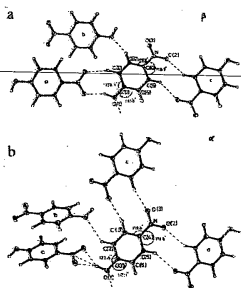
Fig. 1. Molecular packing diagrams of the (a) \beta polymorph of p -nitrophenol, (b) a polymorph of p -nitrophenol, showing 30% probability displacement ellipsoids [37], reproduced with the permission of the American Chemical Society.
