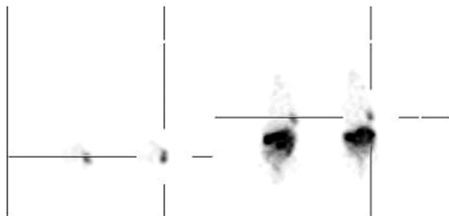
FIGURE 5. Iteratively reconstructed transaxial (left) and coronal (right) PET images of 2 AR42J tumor-bearing nude mice 1 h after injection of 15 pmol (0.49 MBq) ^{68}\text{Ga} -BZH3. Tumors are located in thoracic wall. Tumor uptake and weight: left animal, 5.3 %ID/g, 200 mg; right animal, 7.0 %ID/g, 128 mg.
