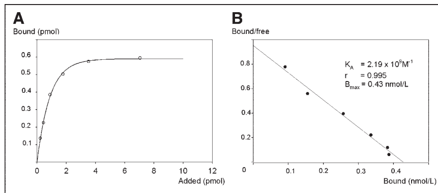
FIGURE 2. Saturation curve (A) and Scatchard transformation (B) of binding of increasing amounts of ^{67}\text{Ga} -BZH3 to 4 \times 10^5 AR42J cells. Cells were incubated for 1 h. Data are means of triplicate samples and are corrected for nonspecific binding ( \leq 3.5\% ).
