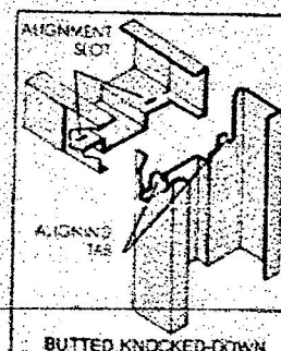
BUTTED KNOCKED-DOWN
