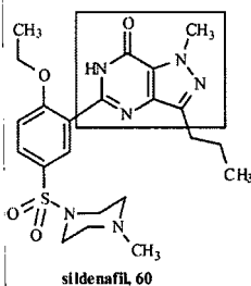
Fig. (2). Examples of ring bioisosterism between drugs belonging to different therapeutic classes.
