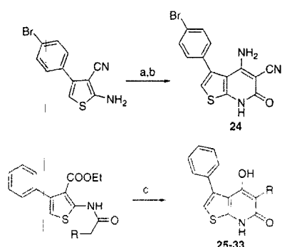
Scheme 3. Reagents and conditions: (a) CH_2(CN)CO_2H , PCl_5 , Et_3N , DCM (90%); (b) NaOEt , EtOH , reflux (43%); (c) NaH , THF, reflux or KHMDS, THF, PhCH_3 , 0 ^{\circ}C –rt, (20–70%).
