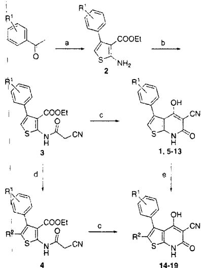
Scheme 1. Reagents and conditions: (a) \text{CH}_2(\text{CN})\text{CO}_2\text{Et} , S, morpholine, EtOH, 60 °C (20–45%); (b) \text{CH}_2(\text{CN})\text{CO}_2\text{Et} , \text{PCl}_5 , \text{Et}_3\text{N} , DCM (90%); (c) NaH, THF, reflux (80%); (d) \text{SOCl}_2 , DCM (90%); (e) \text{C}_5\text{H}_5\text{NHBt}_3 , AcOH or NCS/NBS, AcOH (30–60%).
