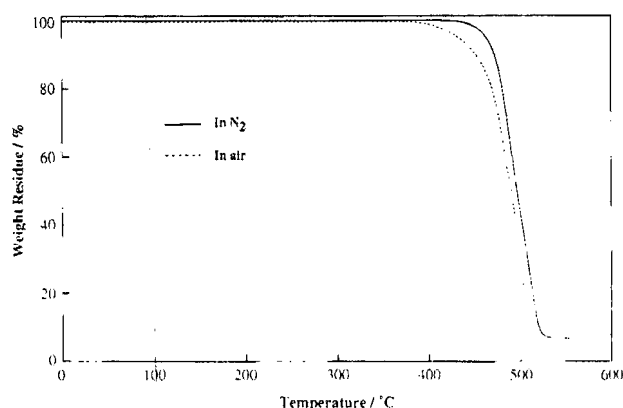
Figure 1. TGA/DTA curves of API-4 in nitrogen and air.
