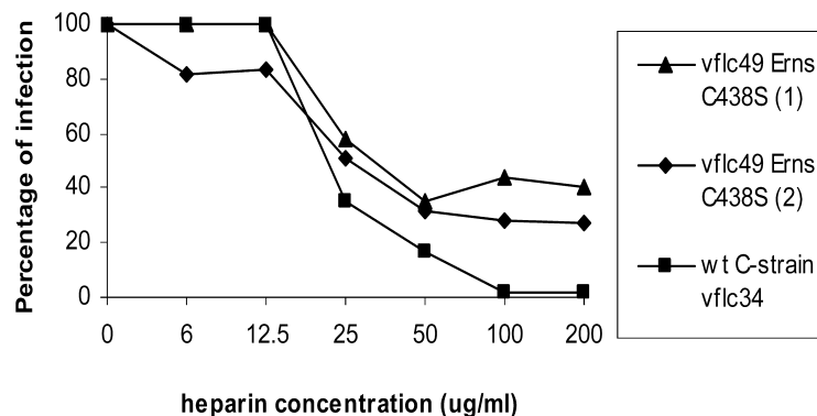
Fig. 3. Dose dependent inhibition of infection of SK6 cells by heparin of mutant virus vflc49 \text{E}^{\text{rns}} C438S (clones 1 and 2), and wt C-strain vflc34 [18]
