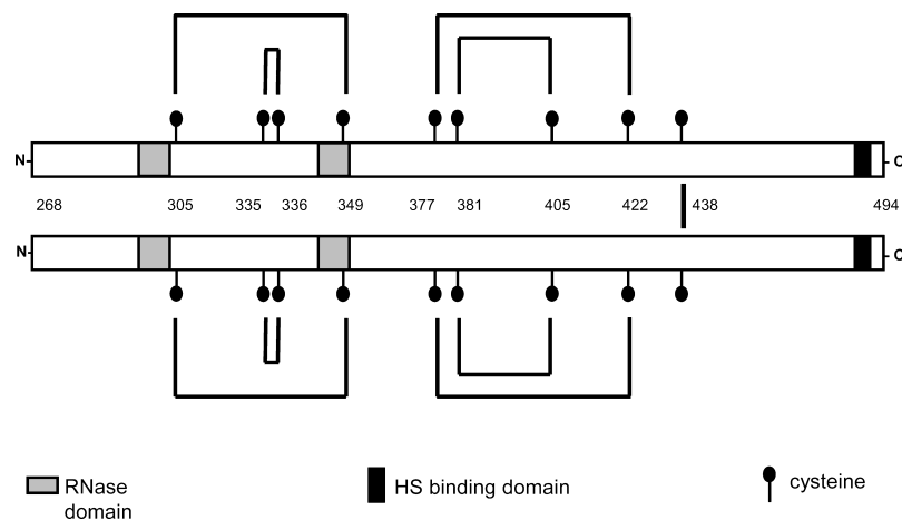
Fig. 1. Schematic representation of the E rns homodimer showing the disulfide bridge connection [13]. Cysteine residues are numbered and the two active RNase domains are shaded. The HS binding domain in the C-terminus of E rns , which was determined for BVDV [10], is depicted as a black box
