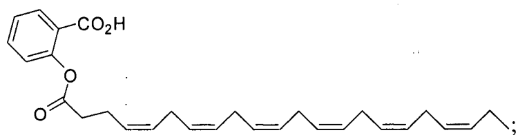
Ia-1
