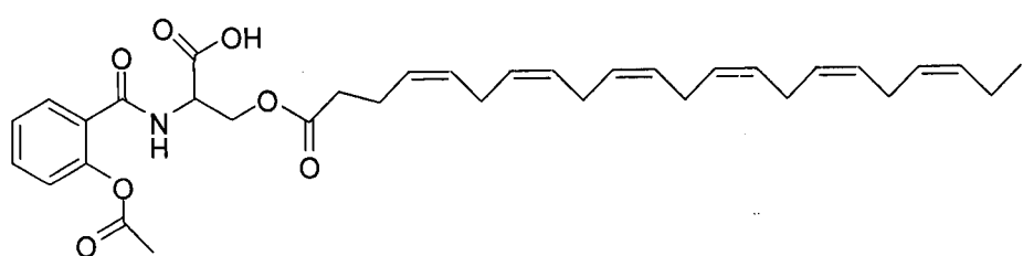
Ic-8
