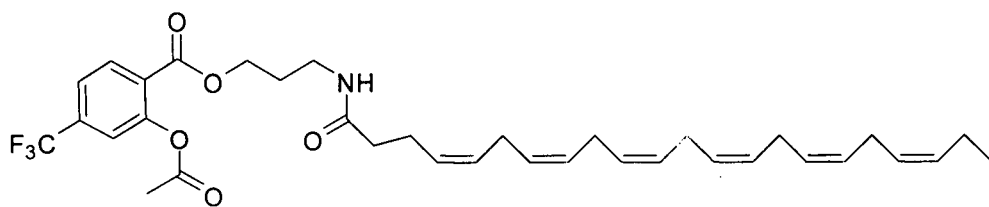
VIb-3
