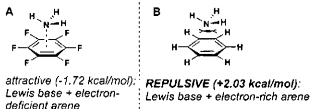
Figure 4. Interaction between a Lewis base (ammonia) which has been calculated to be attractive (A) when the arene is electron deficient and to be repulsive (B) when the arene is electron rich. Interaction energy calculated at the MP2/aug-ccpVDZ/B3LYP 6-311G(d) level. 11
