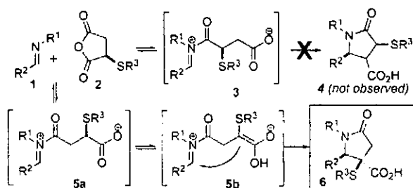
Scheme 1. Reversibility of the Imine–Anhydride Reaction
