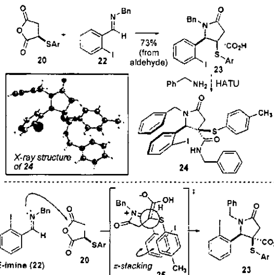
Scheme 1. Synthesis of 24 and Establishment of the Relative Stereochemistry by X-ray Crystallography
