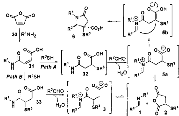
Scheme 3. Mechanism of the One-Pot, 4CR a
