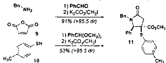
Scheme 2. One-Pot, Four-Component Reaction (4CR)
