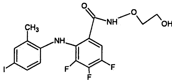
3,4,5-trifluoro-N-(2-hydroxyethoxy)-2-[(4-iodo-2-methylphenyl)amino]benzamide
