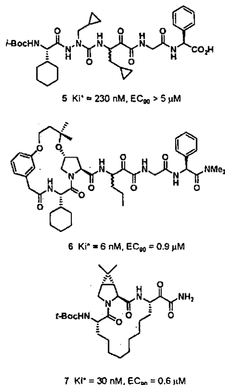
FIGURE 7. Efforts toward depeptization of HCV protease inhibitors.
