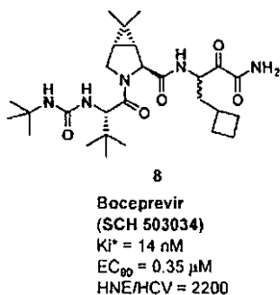
FIGURE 8. HCV protease inhibitor 8 .
