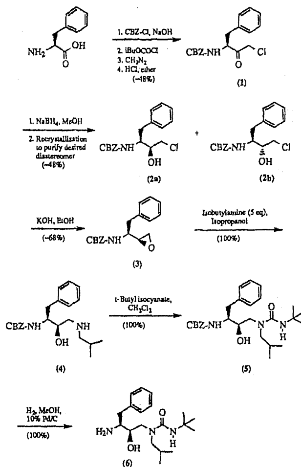
Scheme I
