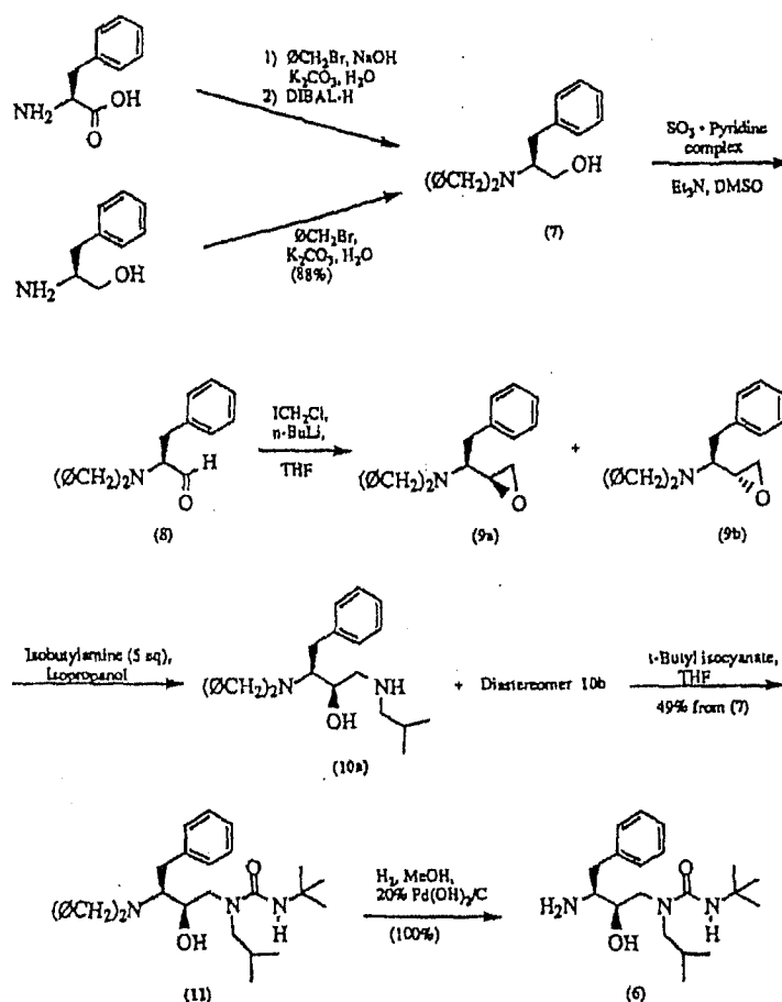
Scheme II
