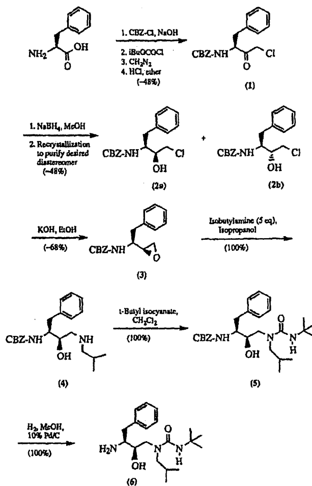
Scheme I
