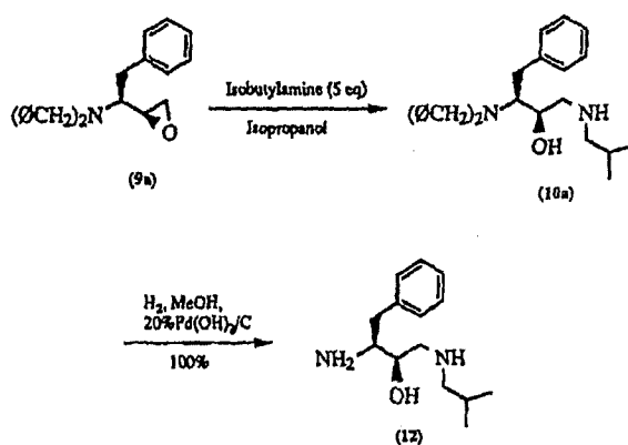
Scheme III
