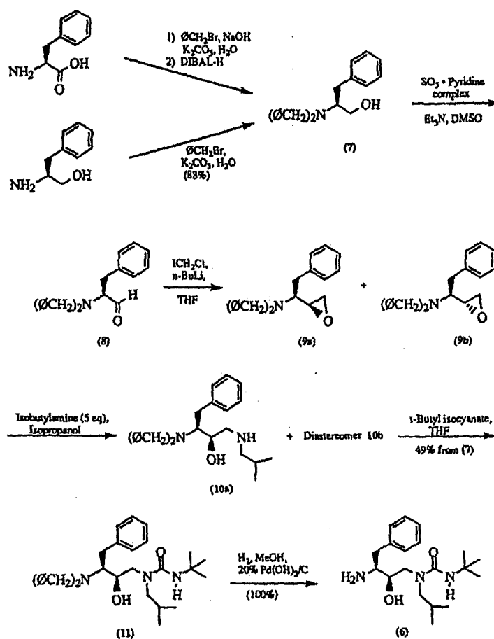
Scheme II
