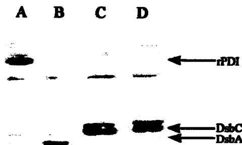
FIG. 2. SDS-PAGE of total cell extracts from cultures coexpressing both tPA and DsbA, DsbC, or DsbA-DsbC. Cells were harvested 3 h after induction and lysed, and equal amounts of total protein from each sample were loaded on a 12% SDS-PAGE gel as described in Materials and Methods. Lanes: A, pBAD-stII-tPA + pLppsOmpArPDI; B, pBAD-stII-tPA + pSE380dsbA; C, pBAD-stII-tPA + pSE420dsbC; D, pBAD-stII-tPA + pSE380dsbAC.
