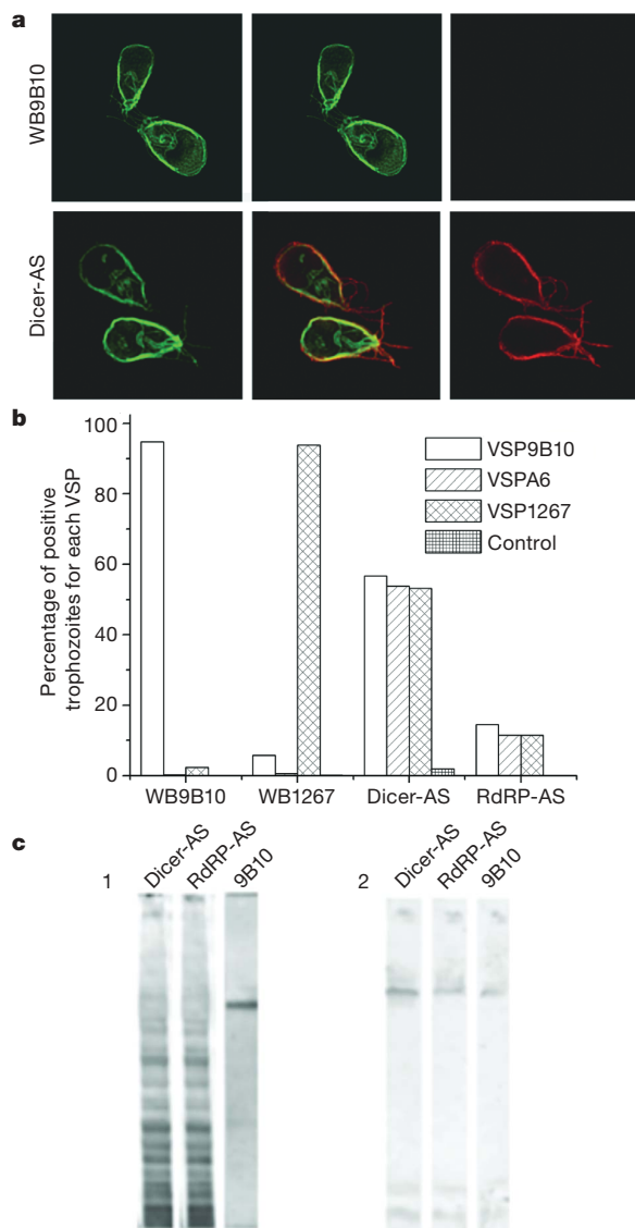
Figure 3 | Expression of different VSPs in Giardia rdp- and dicer-knockdown transgenic trophozoites. a , Direct immunofluorescence assay on mock-transfected (top panel) or Dicer-AS-transfected (bottom panel) trophozoites with FITC-conjugated monoclonal antibody 9B10 (VSP9B10; left panel) and TRITC-conjugated monoclonal antibody 5C1 (VSP1267; right panel). When Giardia Dicer expression was knocked down, trophozoites expressing VSP9B10 on the surface also expressed VSP1267 (merged image; middle panel). b , Percentage of Giardia trophozoites expressing a particular VSP as determined by flow cytometry assays using specific monoclonal antibodies (VSP9B10, monoclonal antibody 9B10; VSP1267, monoclonal antibody 5C1; VSPA6, monoclonal antibody 6A7) on clone WB9B10, clone WB1267, and with cells transfected with antisense constructs for Giardia RdRP (RdRP-AS) or Giardia Dicer (Dicer-AS). Goat anti-mouse immunoglobulins were used as a negative control. Clones display clear single-VSP expression patterns, whereas RdRP-AS and Dicer-AS show expression of more than one VSP per trophozoite. c , Western blot analysis of protein extracts from wild-type WB9B10 and WB9B10 trophozoites in which Dicer has been knocked down. After electrophoresis and transfer to nitrocellulose, the filters were hybridised with either (1) the monoclonal antibody 12F1 clone G3 (generated against the CRGKA domain conserved in all VSPs) or (2) monoclonal antibody 9B10 (specific for VSP9B10). Results show that the specific monoclonal antibody anti-VSP9B10 recognizes only one band in clone WB9B10 and in transgenic trophozoites, whereas the monoclonal antibody 12F1 reacts with many protein species in the transgenic cells, indicating that many VSPs are expressed simultaneously in Giardia when the RNAi pathway has been disrupted.
