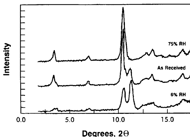
Fig. 5. Powder X-ray diffraction patterns of BMS-180431 magnesium salt as received for testing and after equilibration at 6 and 75% R.H.
