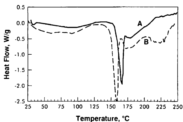
Fig. 4. DSC scans of arginine (A) and lysine (B) salts of BMS-180431 as received for testing.
