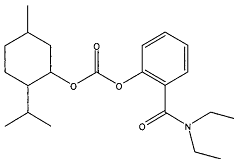
2-(diethylcarbamoyl)fenil 2-isopropil-5-metilciclohexil carbonato
