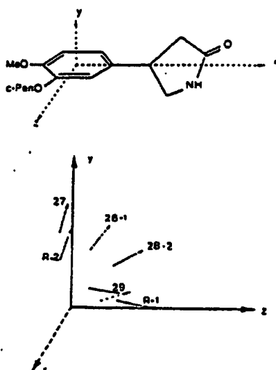
Figure 3. Graphic representation of carbonyl dipole traces of rolipram analogues in the YOZ plane: R-1 and R-2 are two singular conformations of rolipram (see text); dotted arrows refer to trequinsin.
