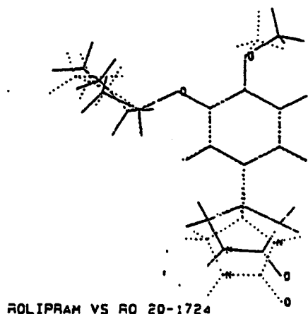
Figure 1. Computer-generated best fits of rolipram (torsion angle \theta = 141^\circ ) and Ro 20-1724 ( 126^\circ and 113^\circ , dashed lines).
