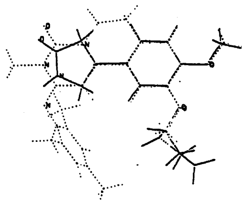
Figure 2. Superposition of rolipram (as compound 6) with trequinsin (dashed lines).
