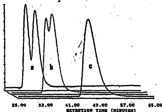
Fig. 3. Effect of temperature on enantiomeric separation of rolipram 1 on Chiralcel-OD. Mobile phase: n -hexane–2-propanol (96:4), 1.0 ml/min, UV detection: 210 nm; temperature: 60°C (a), 40°C (b) and 20°C (c).
