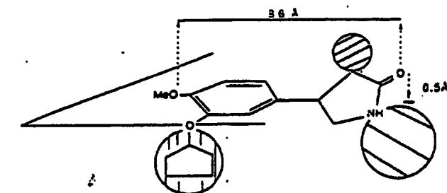
Figure 4. Structural and topological requirements associated with vascular smooth muscle cAMP-PDE inhibitors deriving from rolipram.
