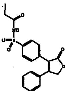
N-[[4-(3-Phenyl-2,3-dihydro-2-oxofuran-4-yl)phenyl]sulfonyl]propanamide
