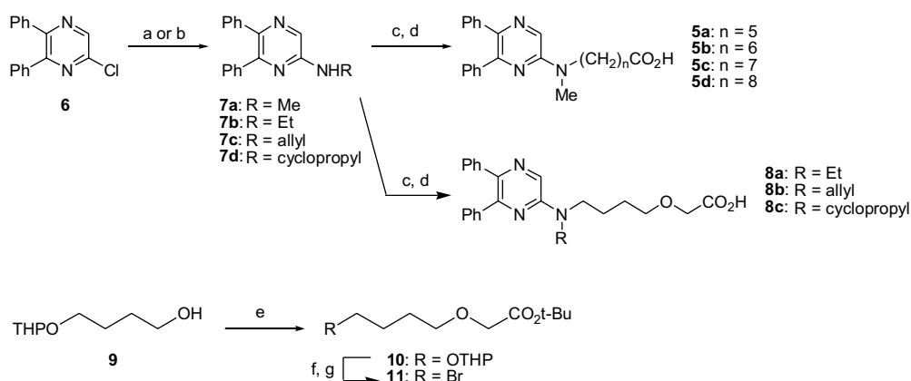
Scheme 1. Reagents: (a) methylamine, MeOH for 7a ; (b) amines, 1-butanol for 7b–d ; (c) i—NaH, DMF; ii—Br(CH 2 ) n CO 2 R for 5a–d , 11 for 8a–c ; (d) 1 N NaOH, MeOH; (e) BrCH 2 CO 2 t-Bu, n -Bu 4 NHSO 4 , aq KOH, benzene; (f) p -TsOH, MeOH; (g) Ph 3 P, CBr 4 , CH 2 Cl 2 .
