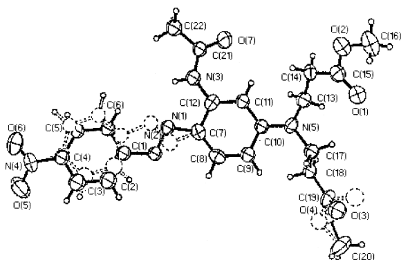
Fig. 5. ORTEP plots of the two molecular conformations (1 and 2) for the X-ray structure determination of 2'-acetamido-4'-[ N,N -bis(2-methoxycarbonylethyl)amino]-4-nitroazobenzene (Scheme I Structure) at 293 K. Thermal ellipsoids are shown at 30% for clarity, with conformer 2 being represented by the solid lines and Conformer 1 by the dotted lines ([48], reproduced with the permission of the American Chemical Society).
