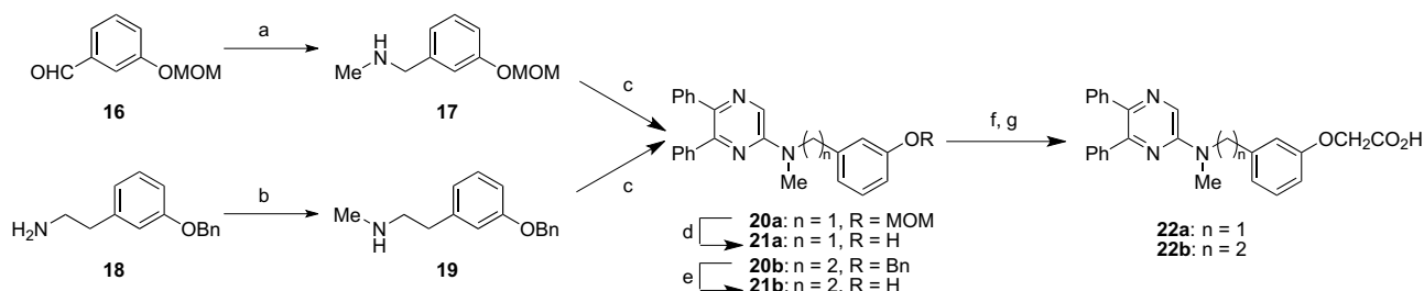
Scheme 3. Reagents: (a) MeNH 2 , H 2 , 5% Pd–C, MeOH; (b) i—HCO 2 Et, EtOH; ii—LiAlH 4 , THF; (c) 6 , K 2 CO 3 , DMF; (d) HCl, MeOH; (e) c -HCl, EtOH; (f) BrCH 2 CO 2 Me, K 2 CO 3 , cat KI, MeCN; (g) 1 N NaOH, MeOH.
