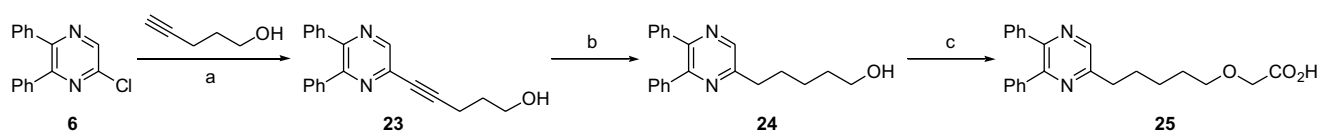
Scheme 4. Reagents: (a) PdCl 2 (PPh 3 ) 2 , CuI, Et 3 N; (b) H 2 , 5% Pd–C, EtOH; (c) i—BrCH 2 CO 2 t -Bu, n -Bu 4 NHSO 4 , aq KOH, benzene; ii—1 N NaOH, MeOH.
