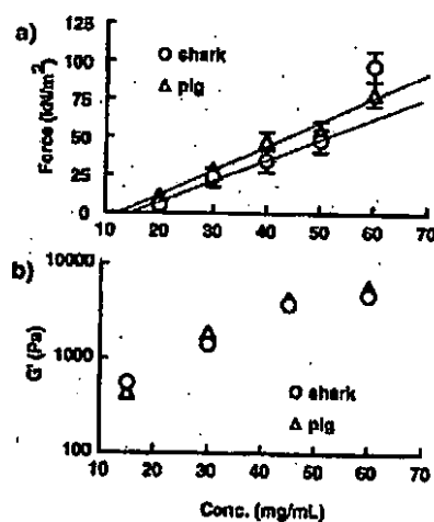
Figure 4. Effect of gelatin concentration on (a) breaking strength and (b) G' of shark and pig gelatin gels (in 0.1 M phosphate buffer, pH 6.0) incubated at 4 °C. Breaking strength was measured by creep meter after 48 h of incubation. Value of G' was measured by rheometer after 2 h of incubation. Conditions of breaking strength: plunger diameter, 5 mm; plunger speed, 5 mm/s. Conditions of rheological study: frequency, 1 Hz; strain, 5%. The bars represent standard deviation of five measurements.
