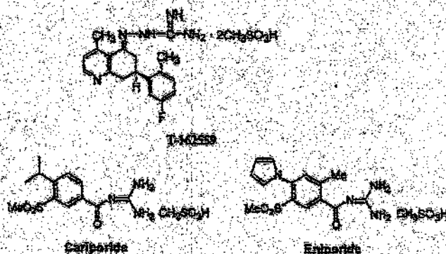
Fig. 1. Chemical structures of T-162559, cariporide, and eniporide.
