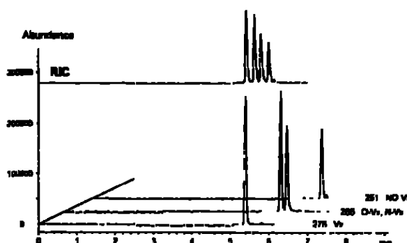
Figure 6. NACE-ESI-MS simultaneous separation of Vx and its three phase I metabolites (1 \mu g/mL each). NACE conditions: running buffer, MeOH-MeCN (20/80 v/v) containing 25 mM ammonium formate and 1 M formic acid; fused-silica capillary, 75 cm total length \times 50 \mu m ID, 360 \mu m OD; pressure injection, 50 mbar for 6 s; applied voltage, 30 kV; temperature, 20°C. MS conditions: SIM positive mode (three ions); capillary voltage, 4 kV; fragmentor, 50 V; drying gas N_2 flow and temperature, 4 L/min and 150°C; nebulizer pressure, 4 psi; sheath liquid, 0.5% formic acid in water-isopropanol (50/50 v/v); sheath flow, 3 \mu L/min. Peak identification as in Fig. 1. For other conditions, see Section 2.2.
