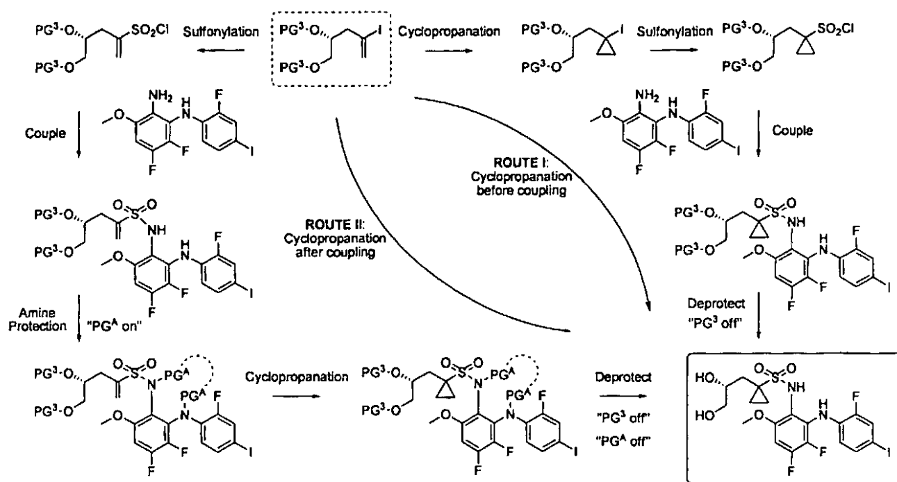
Scheme 2a: (R)-N-(3,4-difluoro-2-(2-fluoro-4-iodophenylamino)-6-methoxyphenyl)-1-(2,3-dihydroxypropyl)cyclopropane-1-sulfonamide
