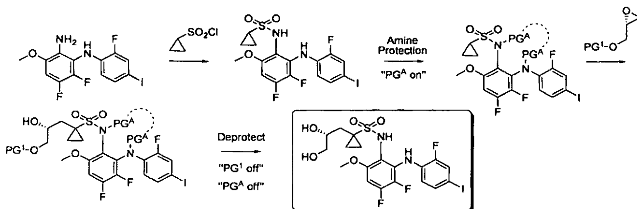
Scheme 5a: (R)-N-(3,4-difluoro-2-(2-fluoro-4-iodophenylamino)-6-methoxyphenyl)-1-(2,3-dihydroxypropyl)cyclopropane-1-sulfonamide
