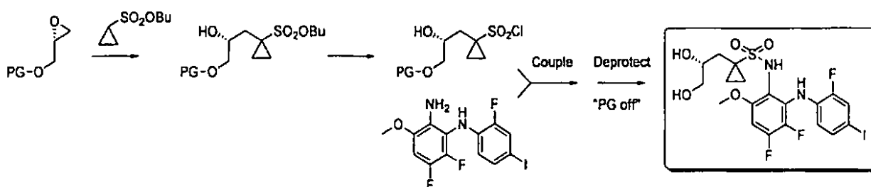
Scheme 4a: (R)-N-(3,4-difluoro-2-(2-fluoro-4-iodophenylamino)-6-methoxyphenyl)-1-(2,3-dihydroxypropyl)cyclopropane-1-sulfonamide
