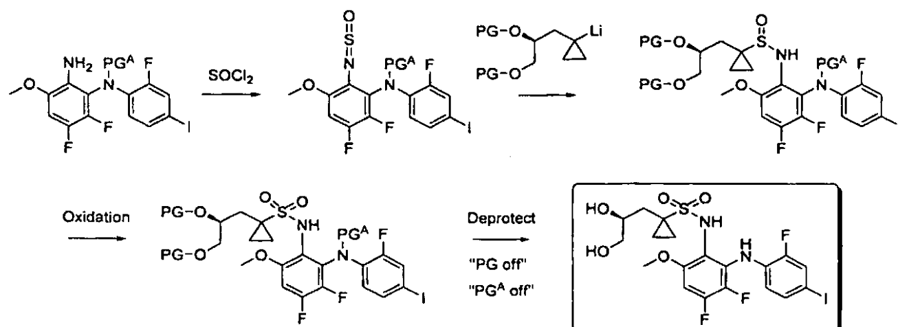
Scheme 6b: (S)-N-(3,4-difluoro-2-(2-fluoro-4-iodophenylamino)-6-methoxyphenyl)-1-(2,3-dihydroxypropyl)cyclopropane-1-sulfonamide
