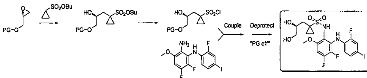
Scheme 4b: (S)-N-(3,4-difluoro-2-(2-fluoro-4-iodophenylamino)-6-methoxyphenyl)-1-(2,3-dihydroxypropyl)cyclopropane-1-sulfonamide
