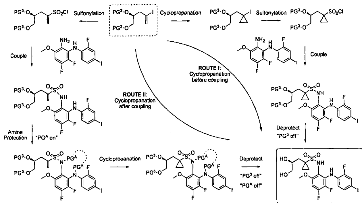
Scheme 2b: (S)-N-(3,4-difluoro-2-(2-fluoro-4-iodophenylamino)-6-methoxyphenyl)-1-(2,3-dihydroxypropyl)cyclopropane-1-sulfonamide
