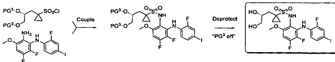
Scheme 7a: (R)-N-(3,4-difluoro-2-(2-fluoro-4-iodophenylamino)-6-methoxyphenyl)-1-(2,3-dihydroxypropyl)cyclopropane-1-sulfonamide
