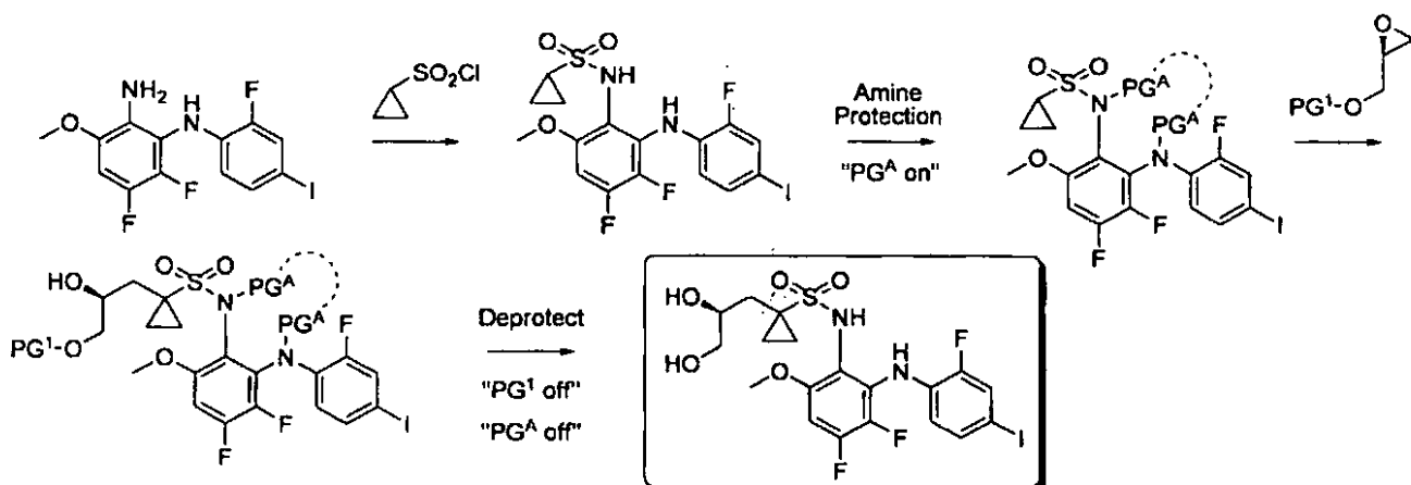
Scheme 5b: (S)-N-(3,4-difluoro-2-(2-fluoro-4-iodophenylamino)-6-methoxyphenyl)-1-(2,3-dihydroxypropyl)cyclopropane-1-sulfonamide
