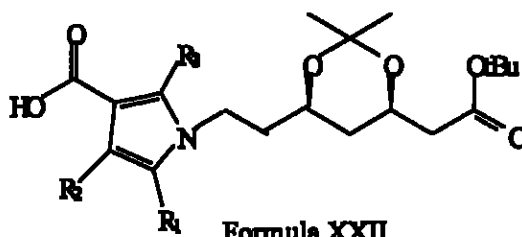
Formula XXII
