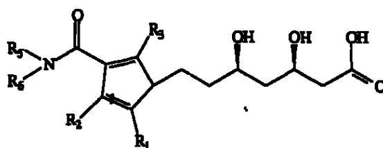
Formula XI
