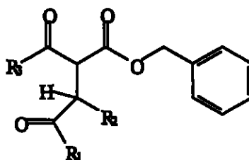
Formula XX
