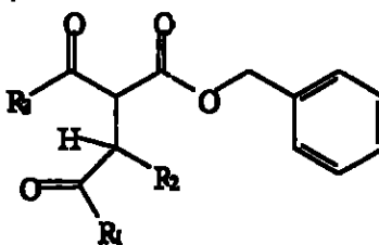
Formula XX
