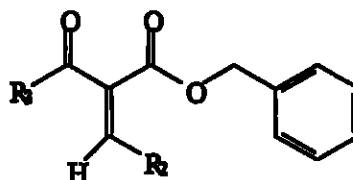
Formula XIX
