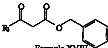
Formula XVIII
