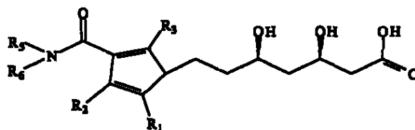
5 Formula XI
