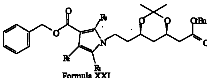
Formula XXI
