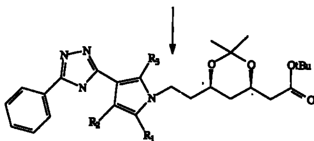
Formula XXIX
