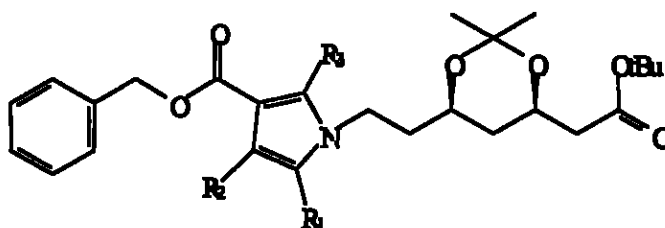
Formula XXI
