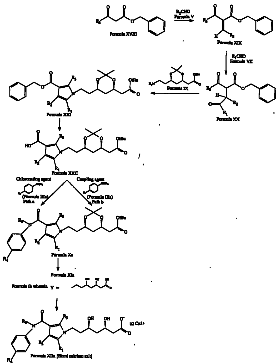
Scheme IIIa
