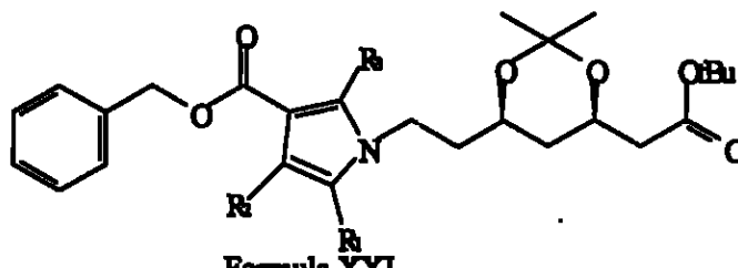
Formula XXI
