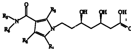
Formula XI
