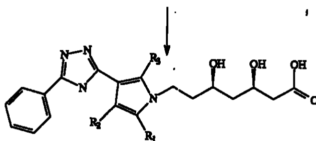
Formula XXX
