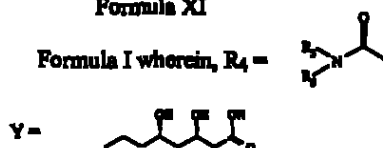
Formula XI
