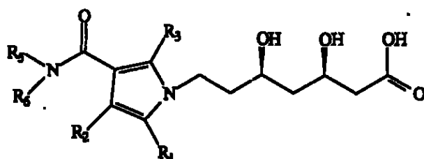
6 Formula XI
