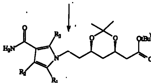
Formula XXVIII
