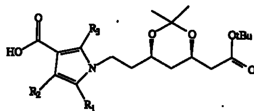
Formula XII
