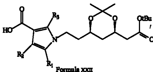
Formula XXII
