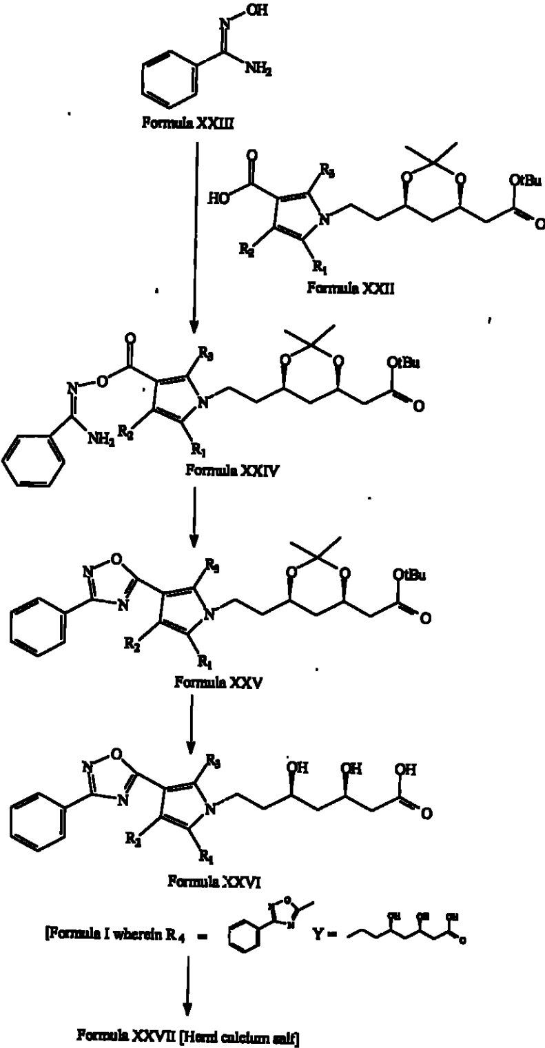
Scheme III
