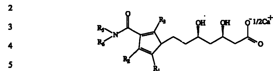
Formula XII
