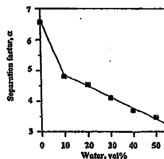
Figure 8. Effect of the water content in the mobile phase on the separation factor \alpha for the reversed phase separation of 3,5-dinitrobenzamidoalanine- N,N -diethylamide enantiomers. Conditions: CSP 10; column, 150 \times 4.6 mm i.d.; mobile phase, acetonitrile-water; flow rate, 1 mL/min.
