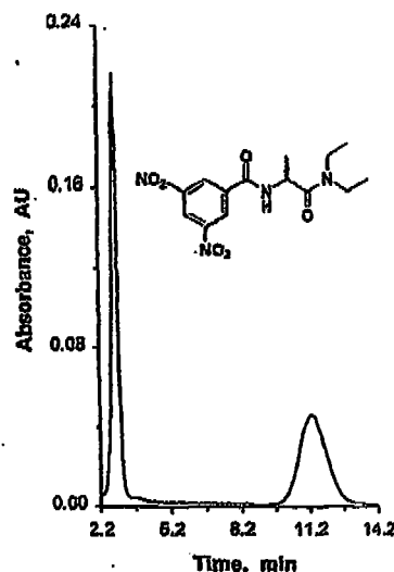
Figure 7. Separation of 3,5-dinitrobenzamidoalanine- N,N -diethylamide enantiomers on chiral stationary phase 10. Conditions: column, 150 \times 4.6 mm i.d.; mobile phase, dichloromethane; flow rate, 1 mL/min.
