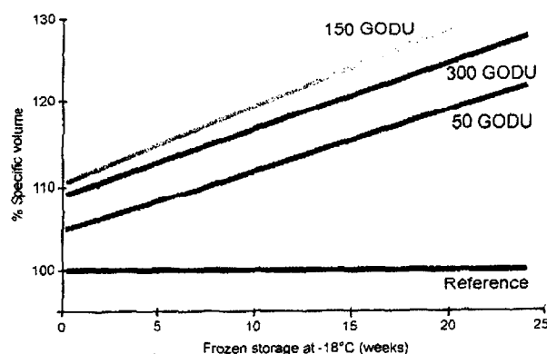
Figure 2.25 Volume of rolls baked from pre-proved frozen dough. Rolls containing glucose oxidase show significantly increased volumes during frozen dough storage and lower rate of deterioration. 30 ppm of a combination of xylanase and fungal alpha -amylase is added to the basic recipe. GODU = units of glucose oxidase/kg flour.
