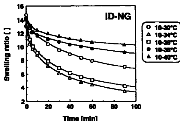
Figure 3. Deswelling kinetics of ID-NG hydrogels from equilibrium swelling condition at 10°C in PBS (pH 7.4) (initial gel dimension: 1.0 mm thick and 15 mm diameter).
