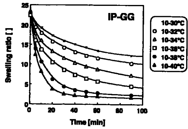
Figure 5 Deswelling kinetics of IP-GG hydrogels from equilibrium swelling condition at 10°C in PBS (pH 7.4) (initial gel thickness = 10 mm thick and 15 mm diameter)
