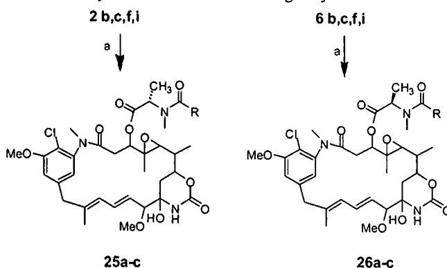
Scheme 7. Synthesis of Thiol-Containing Maytansinoids a
