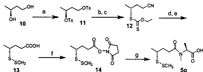
Scheme 4. Synthesis of N -Methyl- N -[(4-( S )-methyldithio)-1-oxopentyl]- S -alanine a
