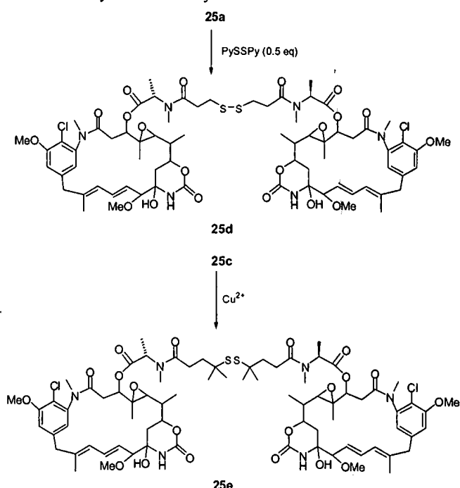
Scheme 9. Preparation of Antibody–Maytansinoid Conjugates a
