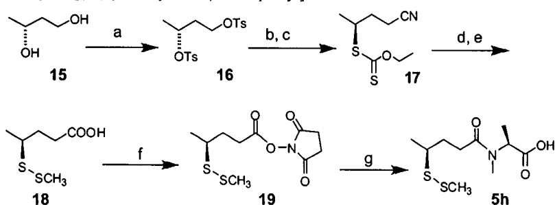
Scheme 5. Synthesis of N -Methyl- N -[(4-( R )-methyldithio)-1-oxopentyl]- S -alanine a
