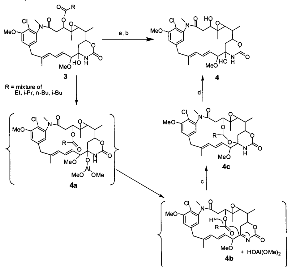
Scheme 1. Synthesis of Maytansinol 19
